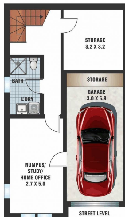
GARDEN LEVEL
