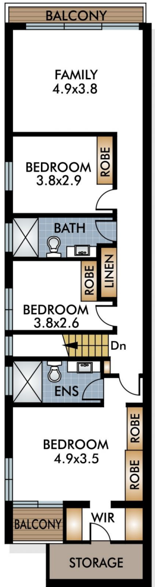
FIRST FLOOR
